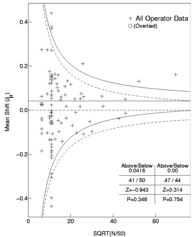
Figure 7. Deployment of 91 individual operator HI – LO mean-shift separations as a function of database size. The inset tables summarize the balance of success of the operator HI – LO performances in the intended directions, compared with both the theoretical chance ( \delta_\mu = 0 ) and composite empirical ( \delta_\mu = 0.0416 ) values.
